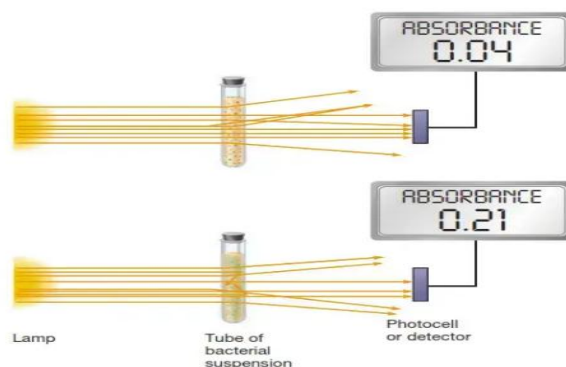
Figure 11. An illustration of turbidity measurement using a spectrophotometer.
