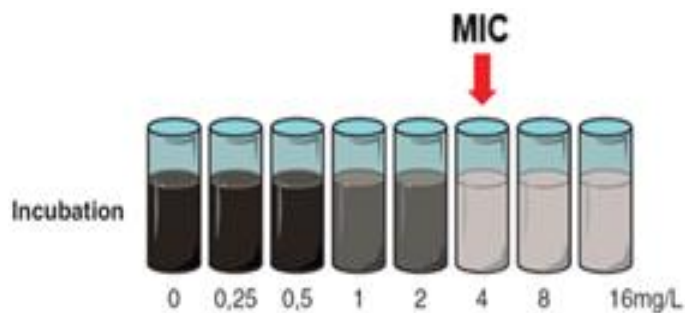
Figure 15. Determination of MIC using broth dilution
