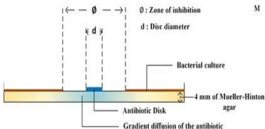
Figure 14. Kirby Bauer disk disc diffusion method
