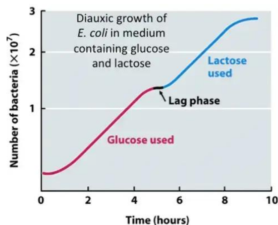
Figure 4. Diauxic growth of bacteria
