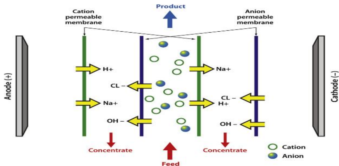
Figure17: Principle of Electro-dialysis.
